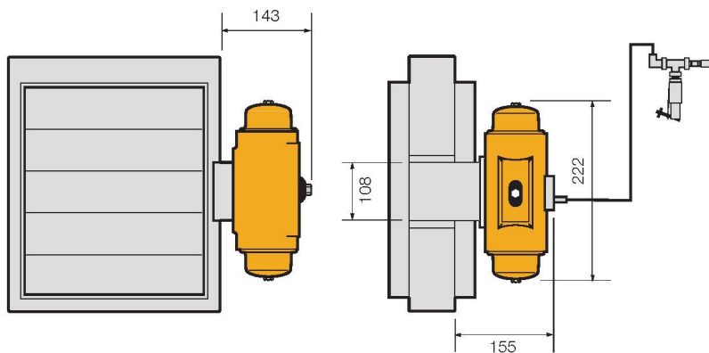
Hytock - 71 (ATEX) Aluminium Switch Box
