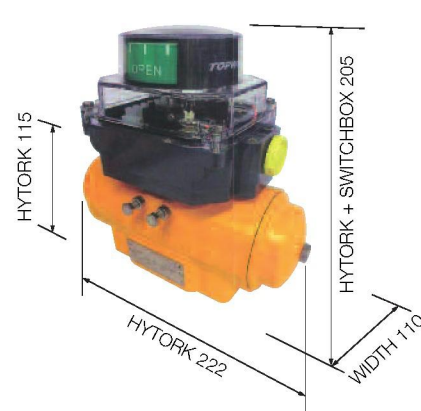
Hytock - 71 (ATEX) Polycarbonate Switch Box
