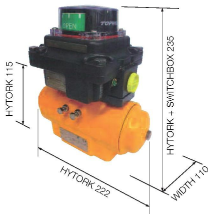
Hytock - 71 (ATEX) Aluminium Switch Box
