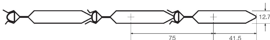
SmokeShield PTC™ blade dimensions
