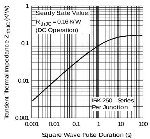
Fig. 11 - Thermal Impedance Z_{\theta JC} Characteristics
