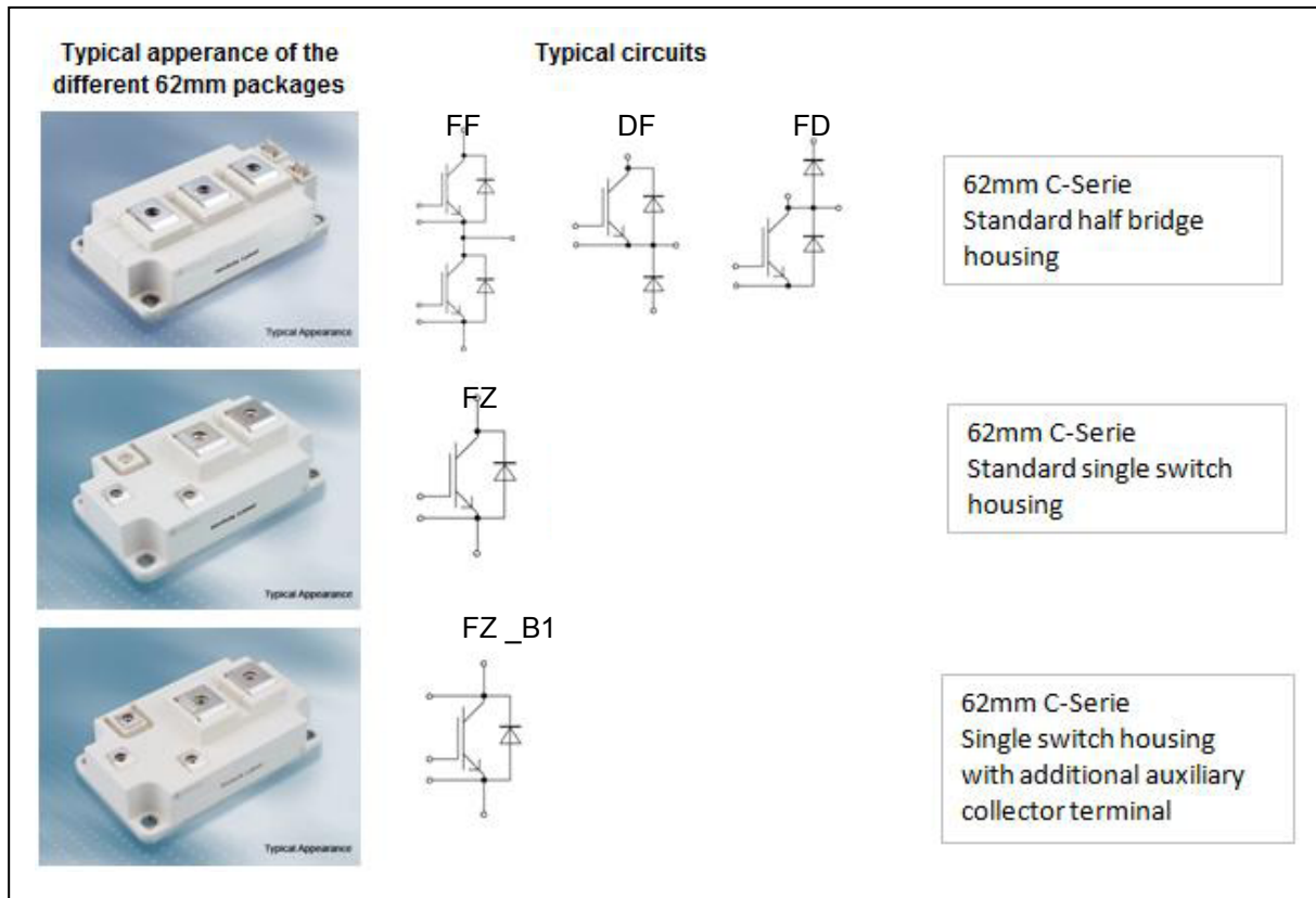
Fig. 2: Typical 62mm module package variants
