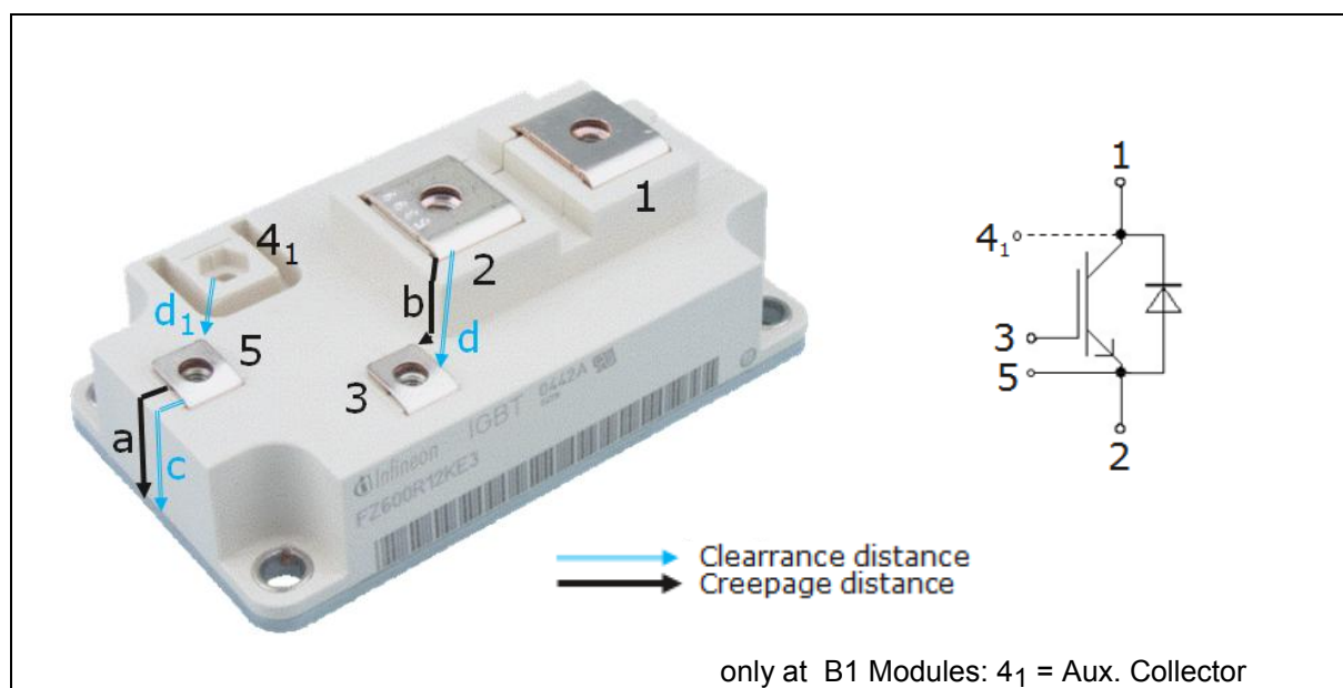
Fig. 4: Shortest creepage distances of the not assembled and unconnected 62mm single switch package
