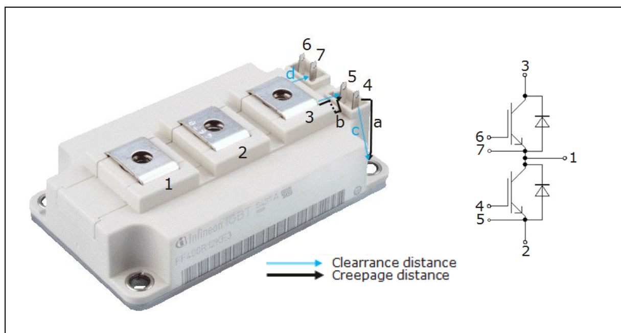
Fig. 3: Shortest creepage distances of the not assembled and unconnected 62mm half bridge package
