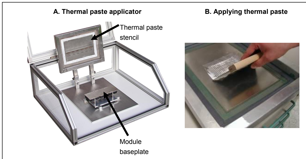
Fig. 8: A. Example of an applicator jig to spread thermal paste in a screen printing process, detailing a module baseplate. B. Application of thermal grease using a stencil
